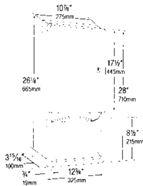
B-4362 CONTURA SERIES PAPER TOWEL DISPENSER Satin-finish stainless steel. Flush tumbler lock. Dispenses 600 C-fold or 800 multifold towels. Rough Wall Opening: 11 3/8" W, 26 1/2" H, 4" min. depth (290 x 675 x 102mm). Av. Mtg. Ht.: 78" (1980mm) to top of unit; Barrier-Free, 59 1/2" (1510mm). Patented.
