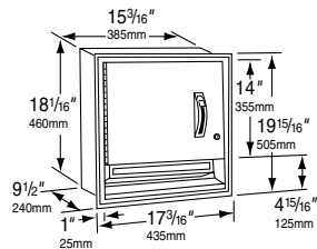
B-3861 CLASSIC SERIES ROLL TOWEL DISPENSER Satin-finish stainless steel. Seamless beveled flange. Delivers preset length of paper towel: 2 1/2", 4" or 5" (65, 100 or 125mm) per stroke. Accepts rolls 8" (205mm) wide, 800 ft (244 m) long. Rough Wall Opening: 16" W, 18 3/4" H, 9 5/8" min. depth (405 x 475 x 245mm). Av. Mtg. Ht.: 70-78" (1780-1980mm) to top of unit; Barrier-Free, 46 1/2" (1180mm).
