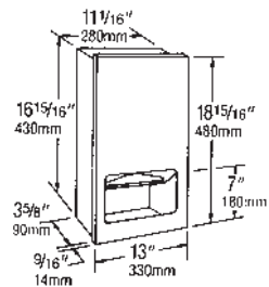
B-35903 TRIMLINE SERIES PAPER TOWEL DISPENSER Satin-finish stainless steel. Door has 90° return, conceals flange. Dispenses 300 C-fold or 400 multifold towels. Rough Wall Opening: 11 1/2" W, 17 3/4" H, 3 3/4" min. depth (290 x 440 x 95mm). Av. Mtg. Ht.: 67" (1700mm) to top of unit; Barrier-Free, 52" (1320mm).
