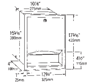
B-359 CLASSIC SERIES PAPER TOWEL DISPENSER Satin-finish stainless steel. Seamless beveled flange. Dispenses 350 C-fold or 475 multifold towels. Door equipped with full-length stainless steel piano-hinge at bottom; swings down for easy filling. Rough Wall Opening: 11 1/4" W, 15 5/8" H, 4" min. depth (285 x 395 x 102mm). Av. Mtg. Ht.: 67" (1700mm) to top of unit; Barrier-Free, 52 1/2" (1335mm).
