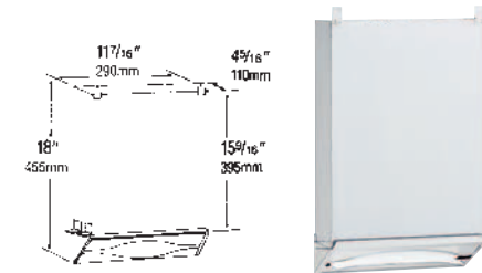
INSTALLED IN WALL OR BEHIND MIRROR
