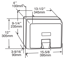
Recessed AirCRAFT Dryers
