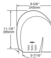
Surface-Mounted B-705 Cub
