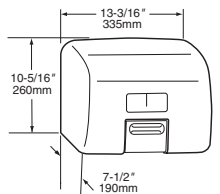
Surface-Mounted B-708 AirGuard, B-709 AirPro
