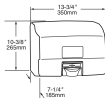
Surface-Mounted AirCRAFT Dryers
