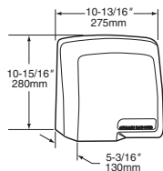
Surface-Mounted B-710 Compac
